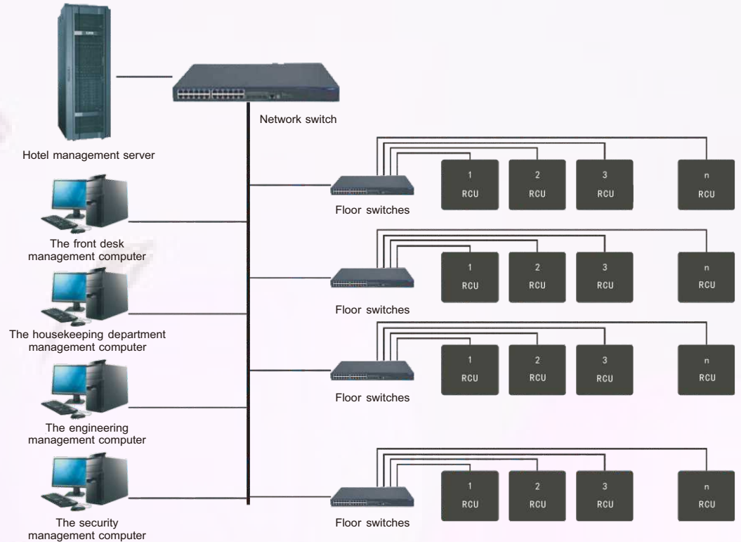
Network diagram
