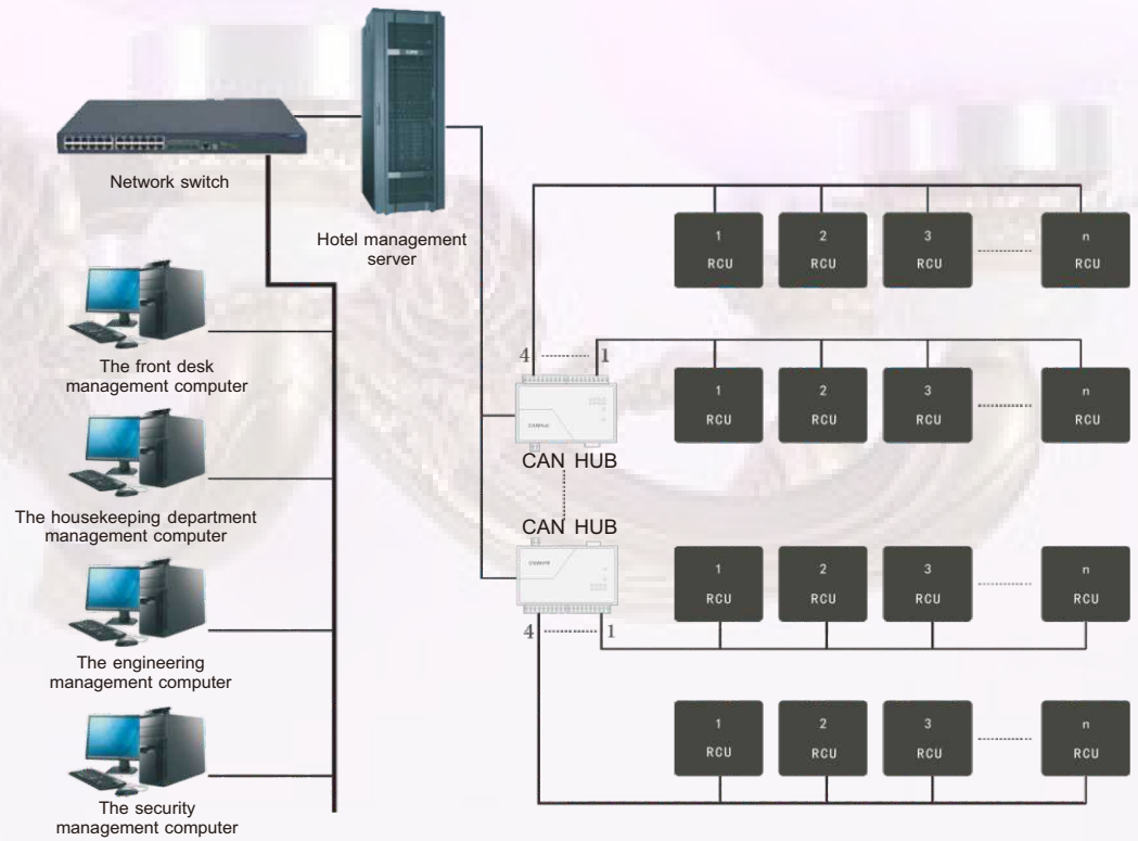
CAN BUS
